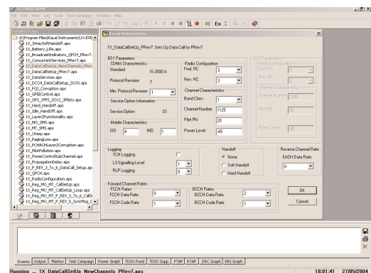
Initial script parameters can be set very easily
