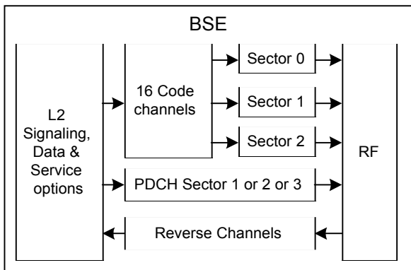
Functional deployment of a BSE
